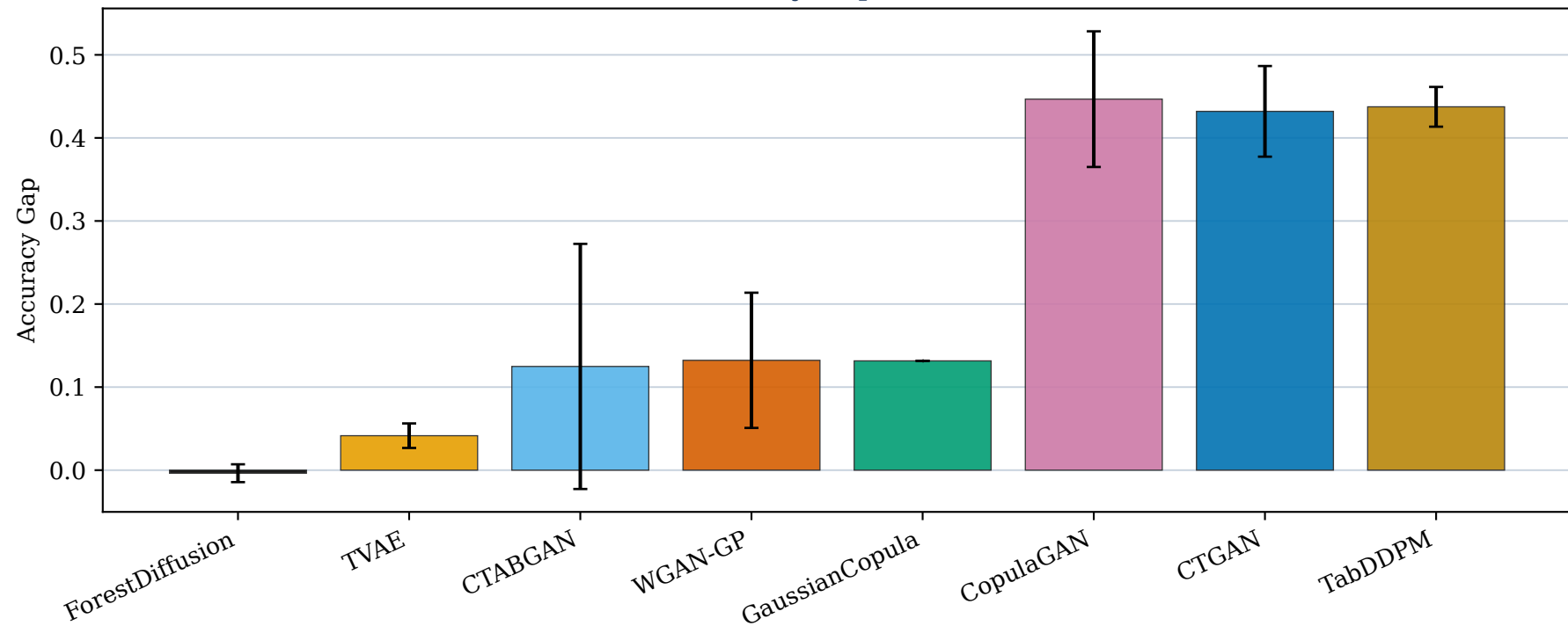
Alzheimer's — Accuracy Gap (mean \pm SD, 10 seeds)
